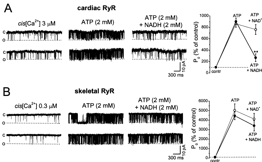
Fig. 3. Effects of NADH and NAD + on cardiac and skeletal RyRs activated by ATP. A: (Left) Cardiac RyR currents in control condition (3 μM cis [Ca 2+ ]), in the presence of 2 mM ATP and subsequent addition of 2 mM NADH. (Right) Changes in P o of cardiac RyRs induced by addition of ATP and by subsequent addition of NADH (filled symbols) or NAD + (open symbols). B: (Left) Skeletal RyR currents in control condition (0.3 μM cis [Ca 2+ ]), in the presence of 2 mM ATP and subsequent addition of 2 mM NADH. (Right) Changes of P o produced by ATP and by subsequent addition of NADH (filled symbols) or NAD + (open symbols). All recordings were made at a holding potential of -20 mV. The dotted line indicated the open channel level. **Statistically different at P < 0.002 compared with ATP alone.
